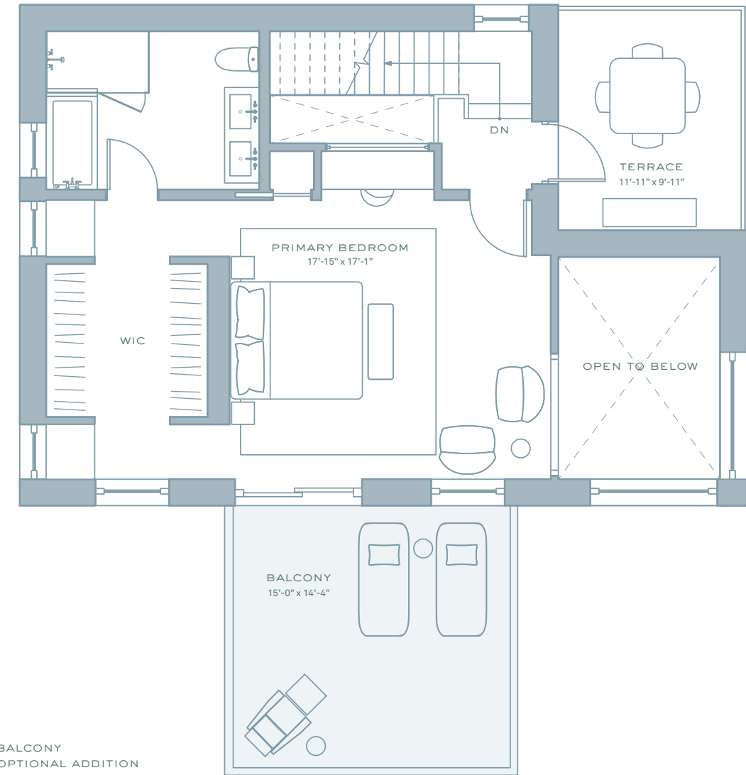
SECOND FLOOR
